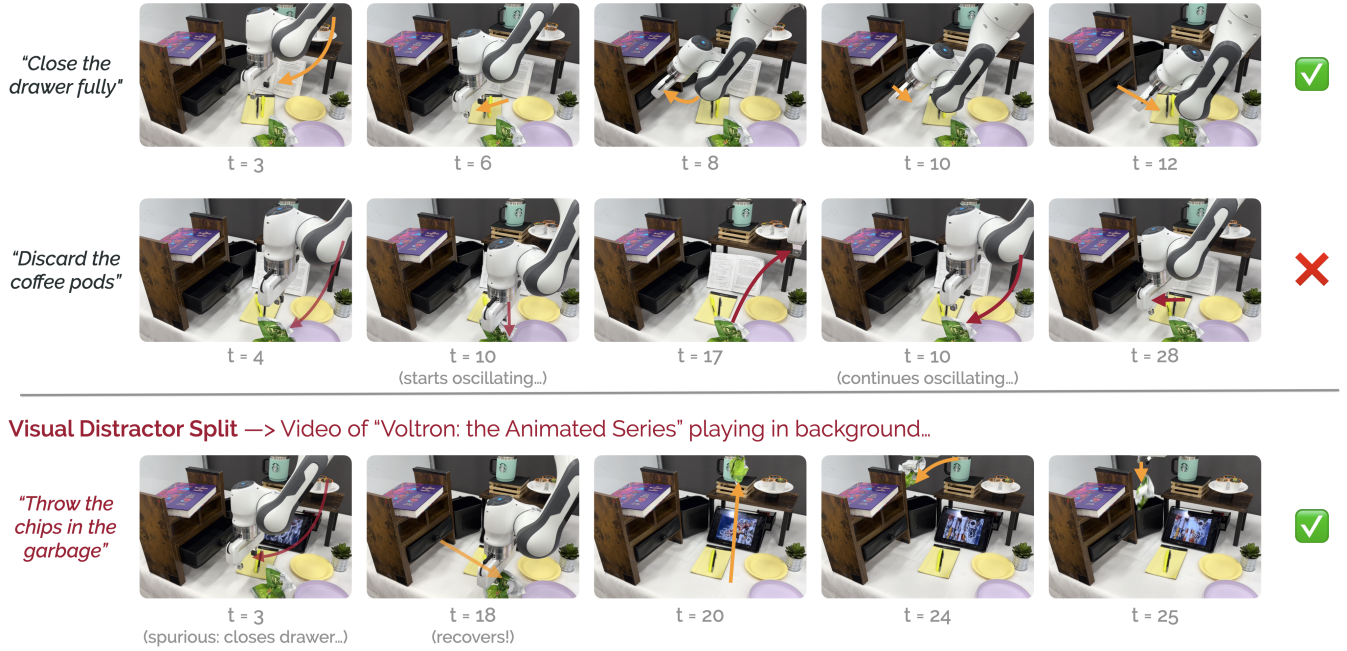
Figure 13: Real-World Language-Conditioned Imitation Rollouts from \mathcal{V} – Gen. We visualize some rollouts from the best-performing real-world language-conditioned imitation learning model, \mathcal{V} – Gen. While some tasks – e.g., discarding the plate of used coffee pods in the trash – prove hard for all methods, \mathcal{V} – Gen shows smooth motion on a series of tasks, even when challenging visual distractors are present. Videos with evaluation rollouts for each method are on our project page .
