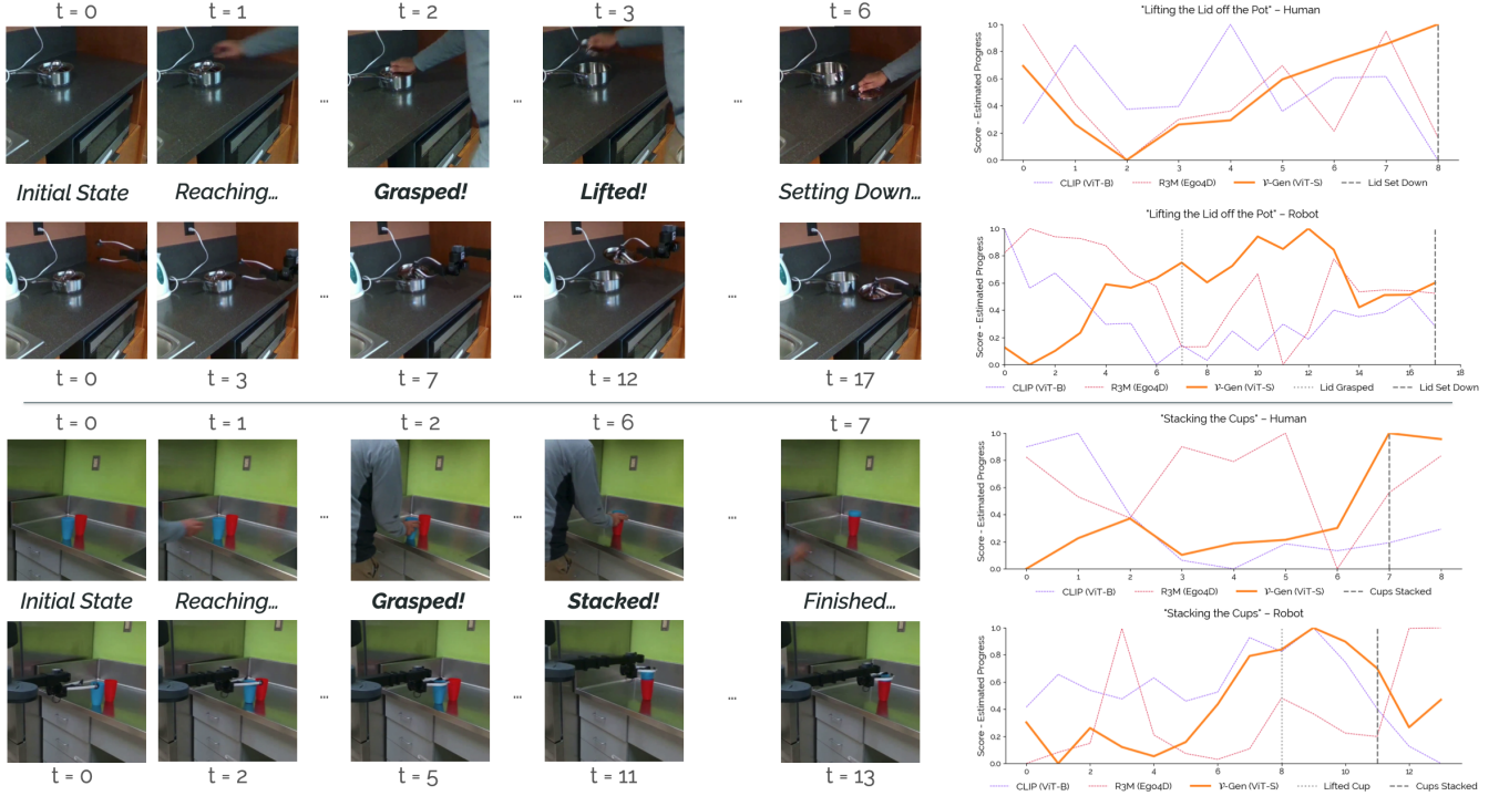
Figure 14: Additional Qualitative Zero-Shot Intent Scoring Examples. Given more videos of humans and robots performing similar behaviors from the WHiRL dataset [Bahl et al. 2022], we evaluate the zero-shot intent scoring capabilities of \mathcal{V} – Gen, R3M (Ego4D) and CLIP (ViT-Base). In general, \mathcal{V} – Gen continues to show a nuanced understanding of semantics over time, in general tracking key points in each video smoothly, whereas both baselines are for the most part predicting random scores.
