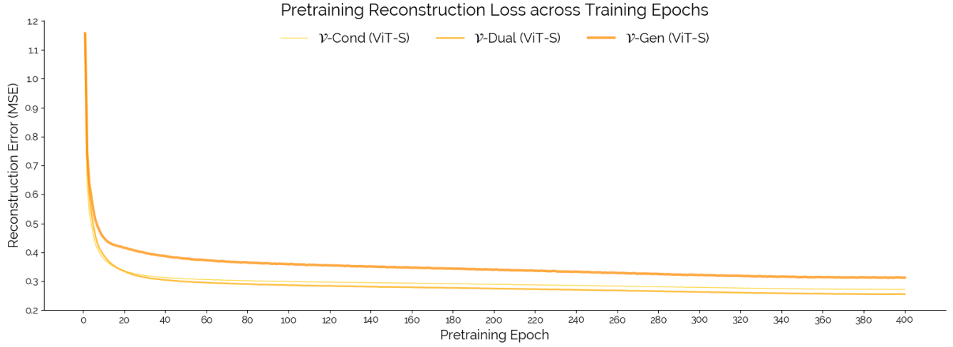
Figure 9: Voltron Pretraining Learning Curves (Reconstruction Error). We visualize the reconstruction error over pretraining epoch for each of the Voltron models. Note that each model learns differently, converging to different reconstruction errors: both the language-conditioned models ( \alpha = 0 ) converge to low reconstruction error, with V – Dual showing that encoding and learning over multi-frame contexts allowing for a better fit. The language generative model V – Gen ( \alpha = 0.5 ) converges to a relatively higher reconstruction error, showing the tension between balancing two disparate objectives.
